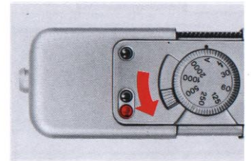
Slow speed check. The signal lights up yellow.
