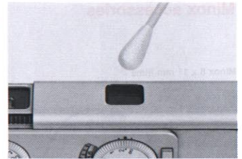
Clean the lens window with a cotton swab – or with a clean rag wound around a matchstick. Slide in the neutral density filter to show up soiling and marks.
